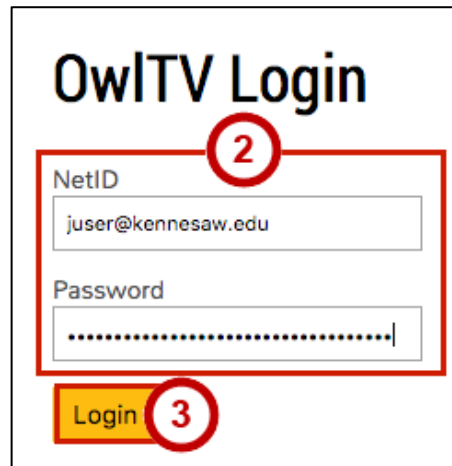
Figure 1 – OwlTV Login
