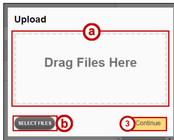
Figure 5 - Upload Files
