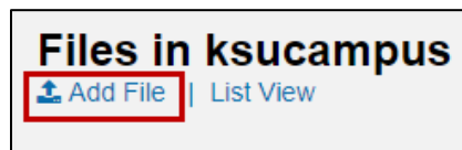
Figure 4 - Add File
