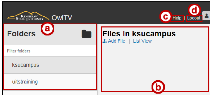
Figure 2 - OwlTV Homepage
